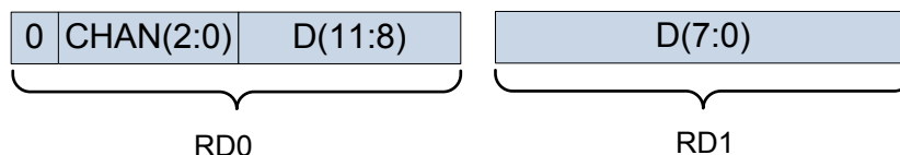
Figure 55 – Channel Data Format
