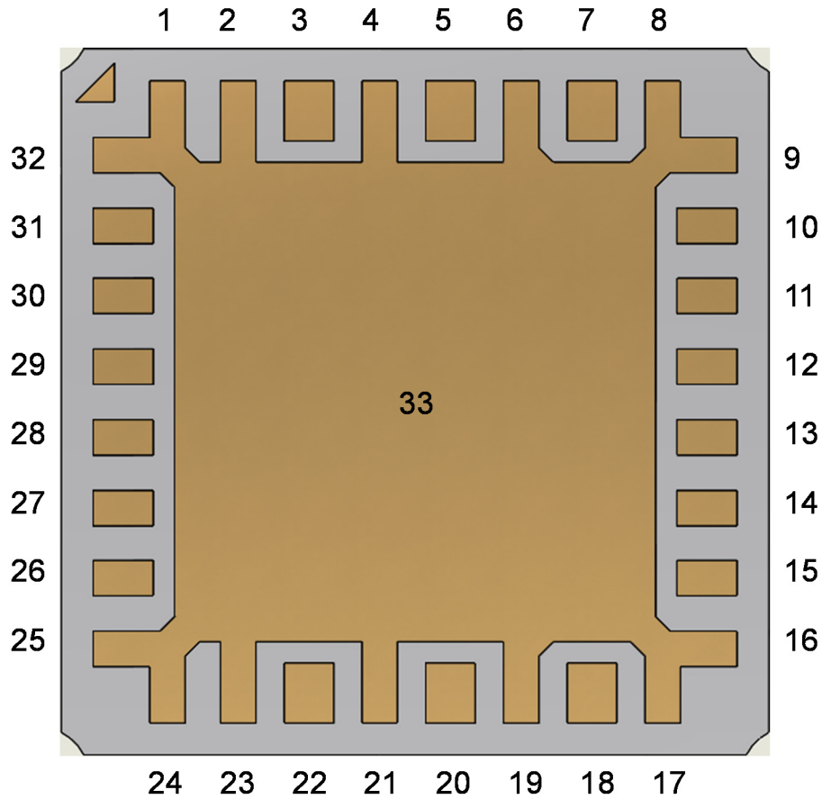
Bottom View
