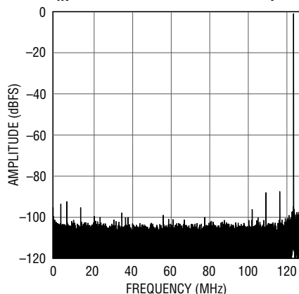
LTC2152-12: 32K Point FFT, f_{IN} = 122\text{MHz} , -1\text{dBFS} , 250Msps
