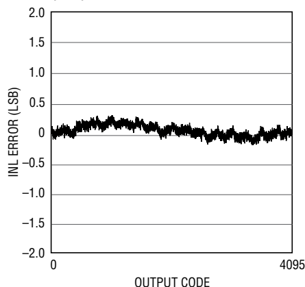
LTC2152-12: Integral Nonlinearity (INL)
