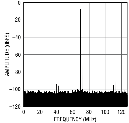
LTC2152-12: 32K Point 2-Tone FFT, f_{IN} = 71\text{MHz} and 69\text{MHz} , 250Mps
