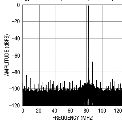
LTC2152-12: 32K Point FFT, f_{IN} = 420\text{MHz} , -1\text{dBFS} , 250Msps
