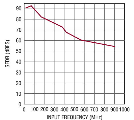
LTC2152-12: SFDR vs Input Frequency, -1\text{dBFS} , 1.5V Range, 250Mps
