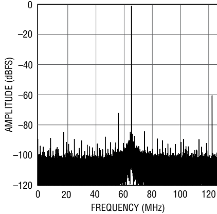
LTC2152-12: 32K Point FFT, f_{IN} = 567\text{MHz} , -1\text{dBFS} , 250Mps
