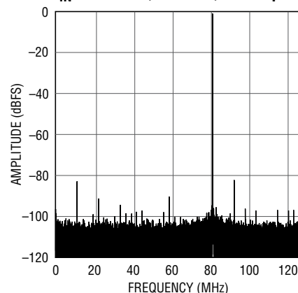
LTC2152-12: 32K Point FFT, f_{IN} = 171\text{MHz} , -1\text{dBFS} , 250Msps
