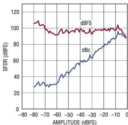
LTC2152-12: SFDR vs Input Level, f_{IN} = 70\text{MHz} , 1.5V Range, 250Mps
