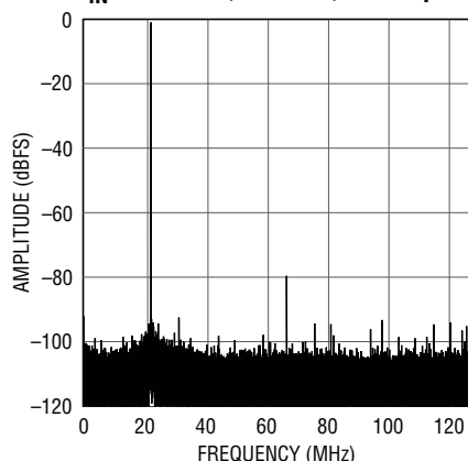
LTC2152-12: 32K Point FFT, f_{IN} = 229\text{MHz} , -1\text{dBFS} , 250Msps
