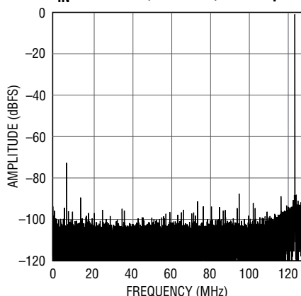
LTC2152-12: 32K Point FFT, f_{IN} = 380\text{MHz} , -1\text{dBFS} , 250Msps
