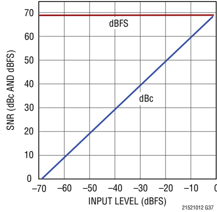
LTC2151-12: SNR vs Input Level, f_{IN} = 70\text{MHz} , 1.5V Range, 210Msps
