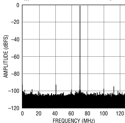
LTC2152-12: 32K Point FFT, f_{IN} = 70\text{MHz} , -1\text{dBFS} , 250Msps
