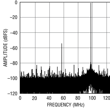
LTC2152-12: 32K Point FFT, f_{IN} = 907\text{MHz} , -1\text{dBFS} , 250Mps
