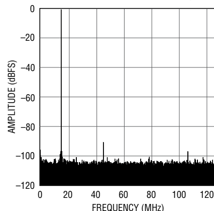
LTC2152-12: 32K Point FFT, f_{IN} = 15\text{MHz} , -1\text{dBFS} , 250Msps
