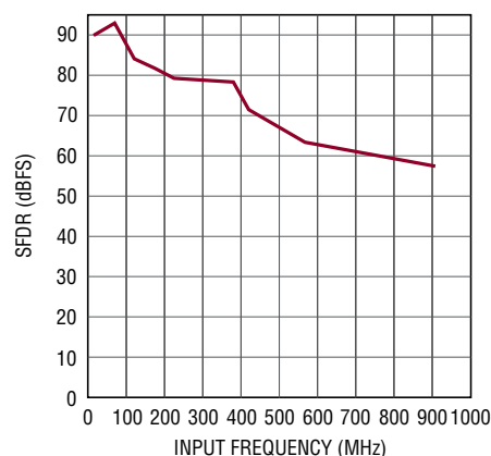
LTC2150-12: SFDR vs Input Frequency, -1dBFS, 1.5V Range, 170Msps
