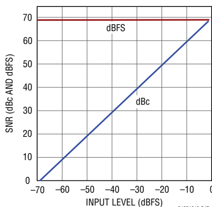
LTC2152-12: SNR vs Input Level, f_{IN} = 70\text{MHz} , 1.5V Range, 250Mps
