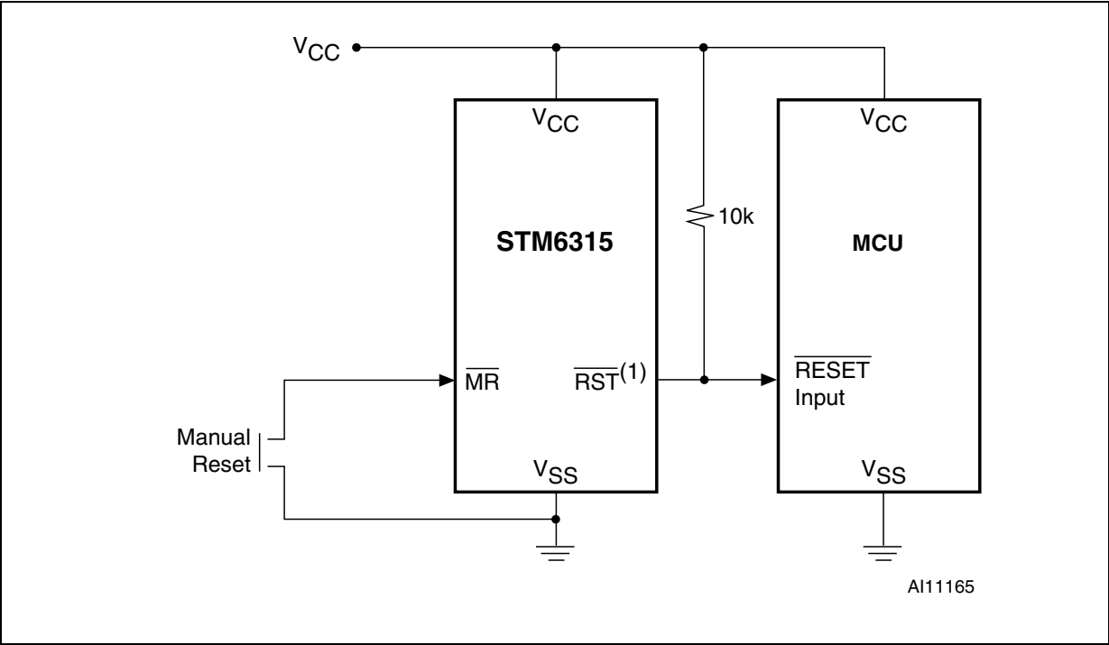
Figure 4. Hardware hookup
