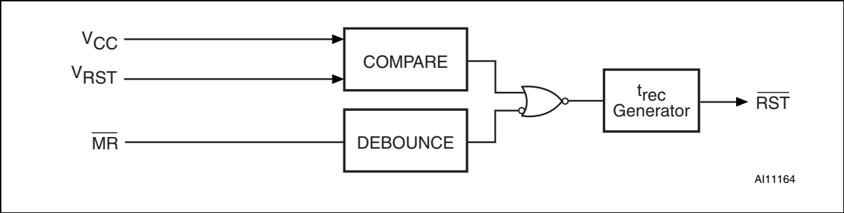
Figure 3. Block diagram
