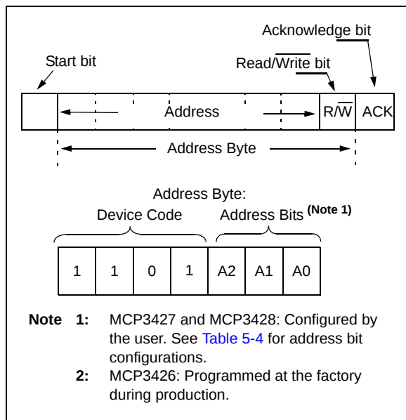
FIGURE 5-1: Address Byte.
