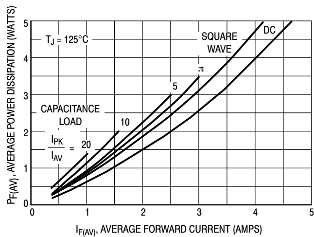
Figure 5. Power Dissipation
