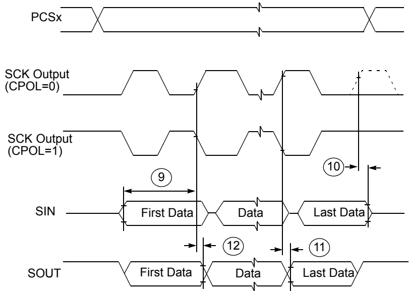
Figure 25. DSPI modified transfer format timing – master, CPHA = 1
