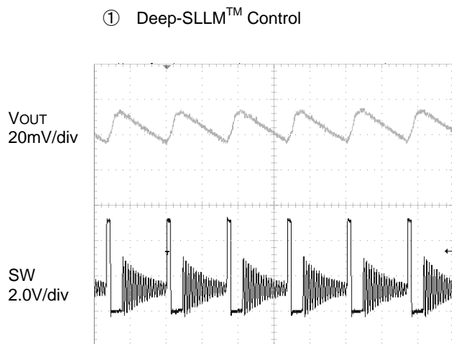
Figure 41. Switching Waveform at Deep-SLLM™ Control (VIN=5.0V, VOUT=1.2V, IOU=100mA)
