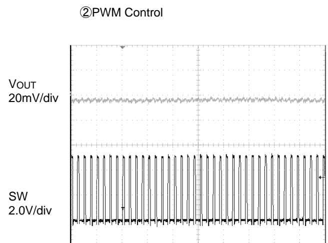
Figure 42. Switching Waveform at PWM Control (VIN=5.0V, VOUT=1.2V, IOU=3A)
