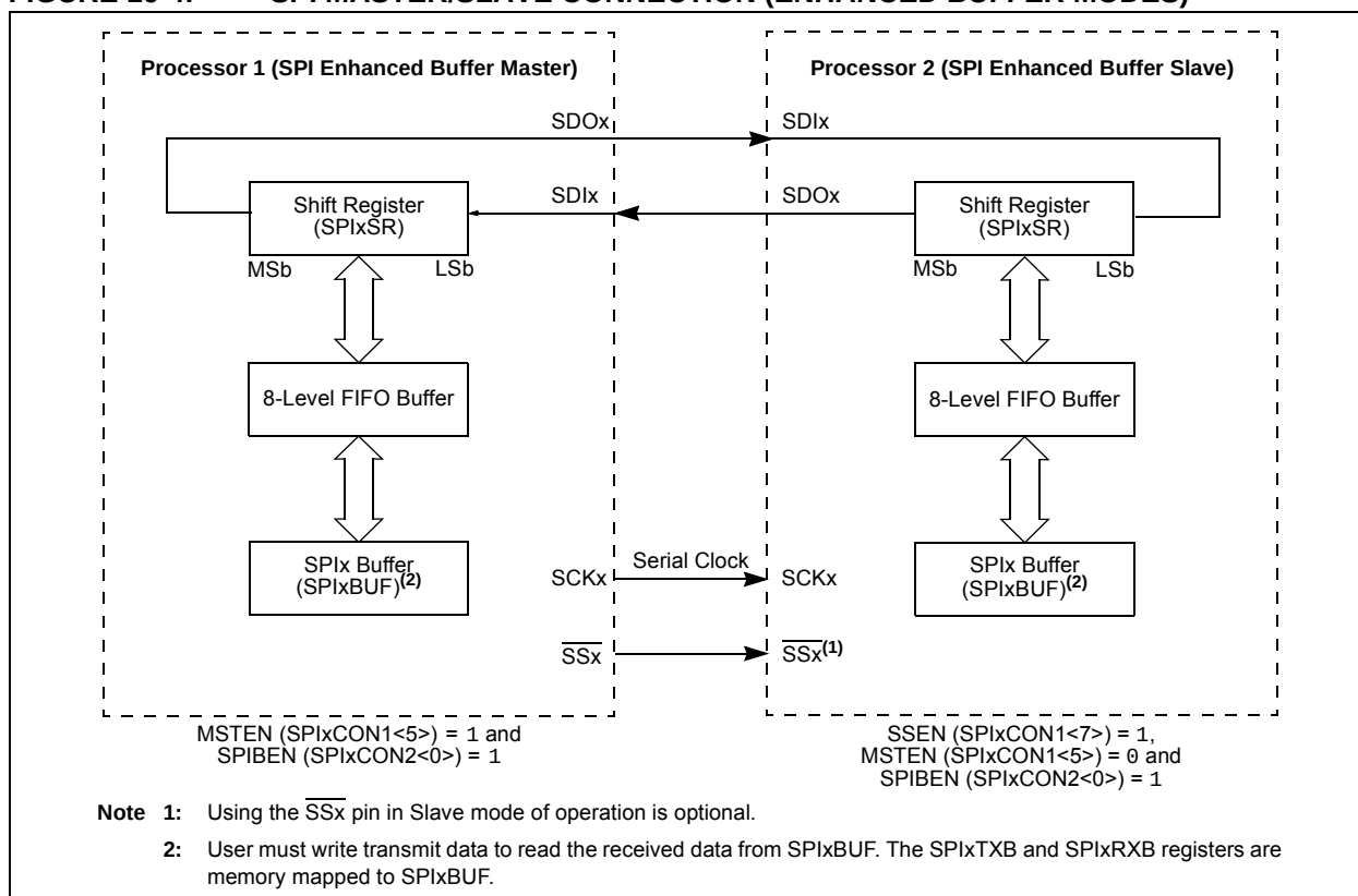
FIGURE 16-4: SPI MASTER/SLAVE CONNECTION (ENHANCED BUFFER MODES)
