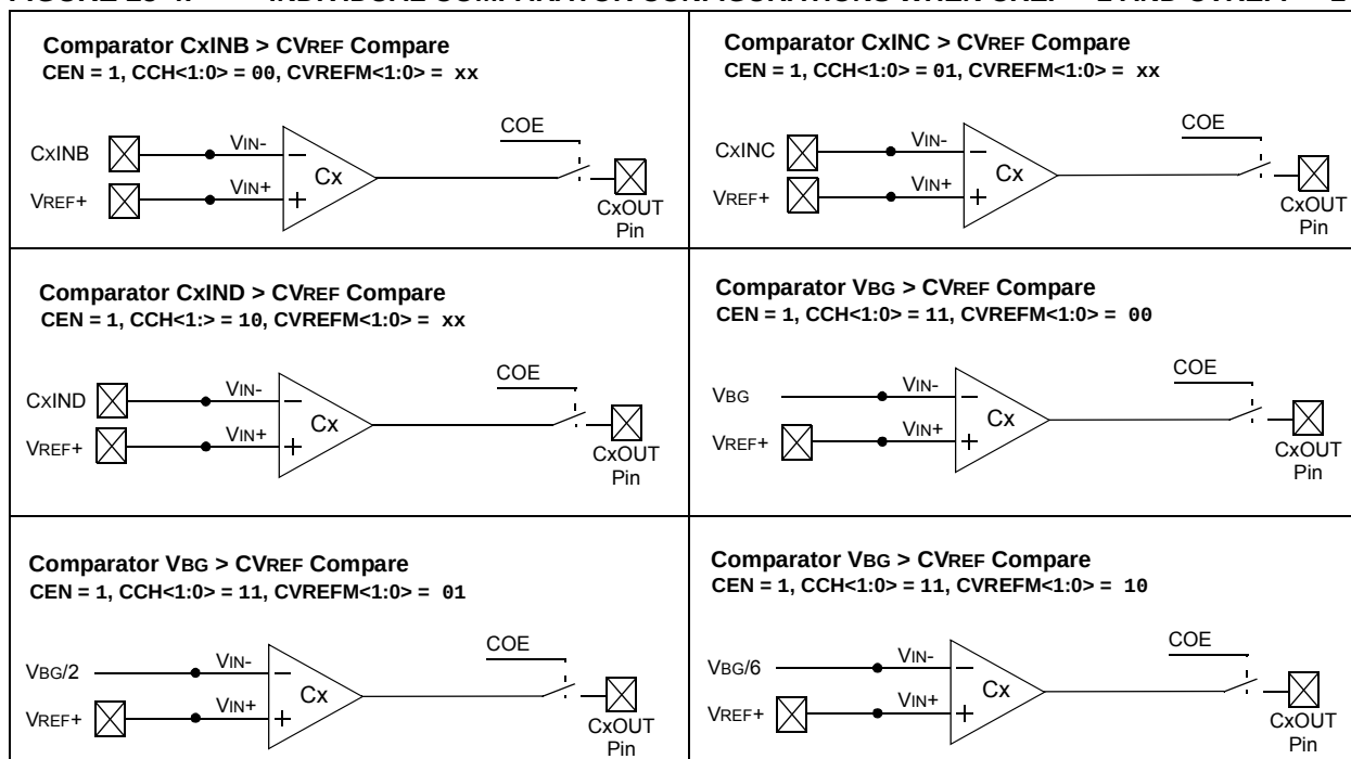
FIGURE 25-4: INDIVIDUAL COMPARATOR CONFIGURATIONS WHEN CREF = 1 AND CVREFP = 1
