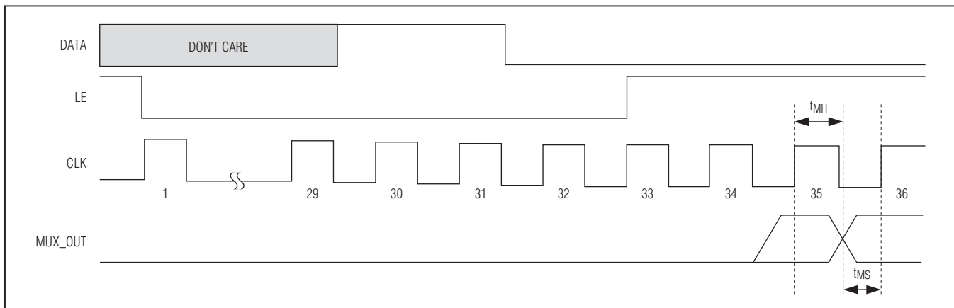
Figure 2. Initiating Readback
