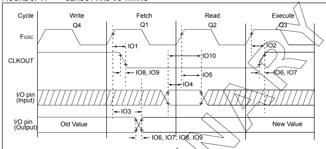
FIGURE 37-7: CLKOUT AND I/O TIMING
