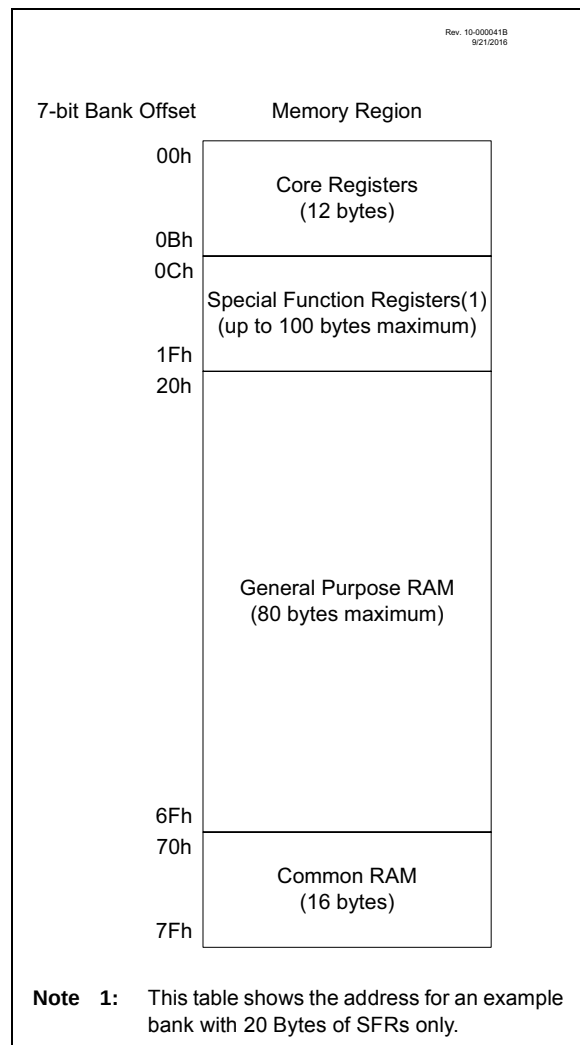
FIGURE 4-3: BANKED MEMORY PARTITIONING
