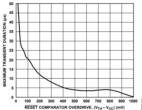
Figure 7. Maximum Transient Duration vs. RESET Comparator Overdrive
