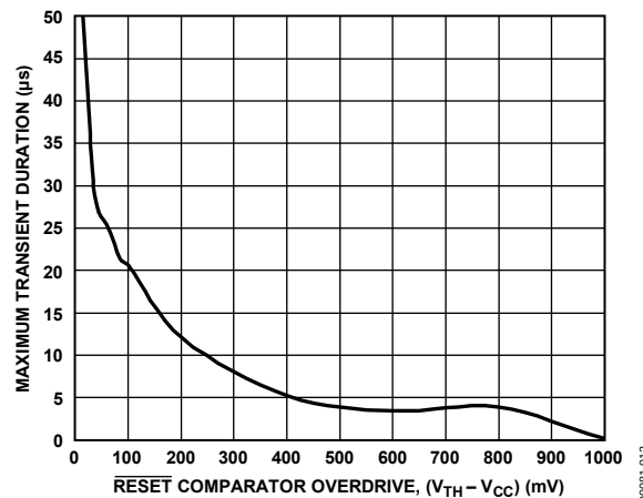
Figure 7. Maximum Transient Duration vs. RESET Comparator Overdrive
