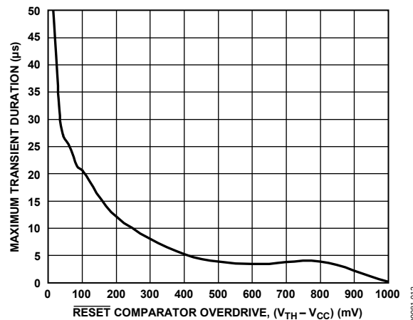
Figure 7. Maximum Transient Duration vs. \overline{RESET} Comparator Overdrive
