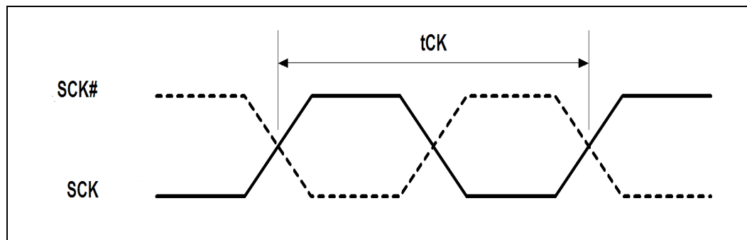
Figure 8-10. Clock Cycle Time
