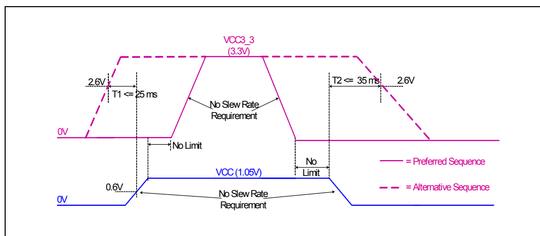
Figure 8-37. Sequencing Requirements between PCH VCC3_3 and VCC Core Rail
