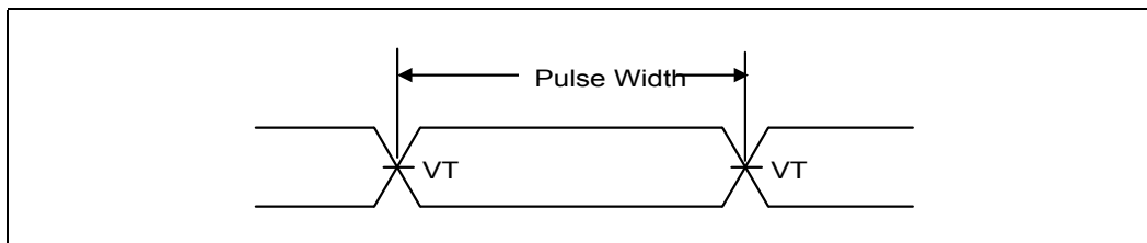
Figure 8-16. Pulse Width
