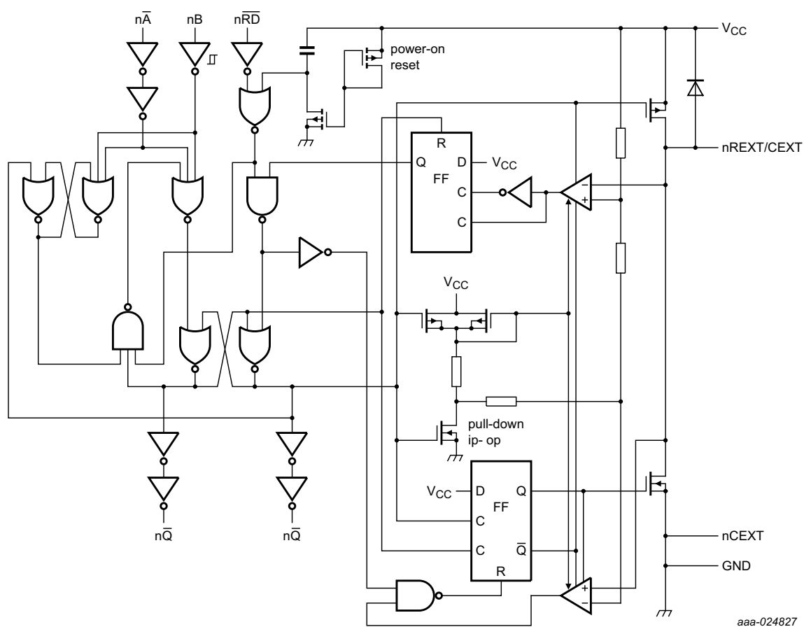
Fig 4. Logic diagram
