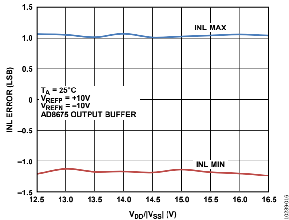
Figure 15. Integral Nonlinearity Error vs. Supply Voltage, \pm 10 V Span
