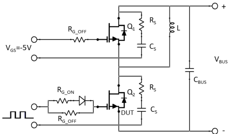
Figure 24. Clamped inductive load switching test circuit An RC snubber ( R_S = 5\Omega and C_S = 330\text{pF} ) is required to improve the turn-off waveforms.
