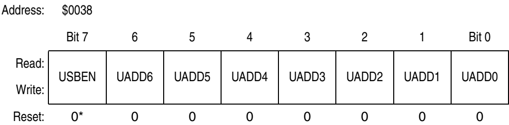
Figure 9-15. USB Address Register (UADDR)
