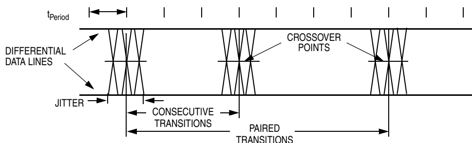
Figure 9-13. Data Jitter
