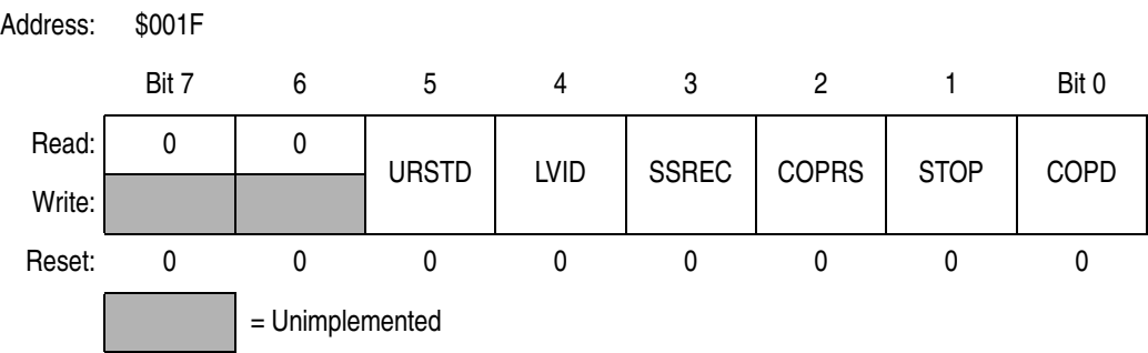
Figure 15-2. Configuration Register (CONFIG)
