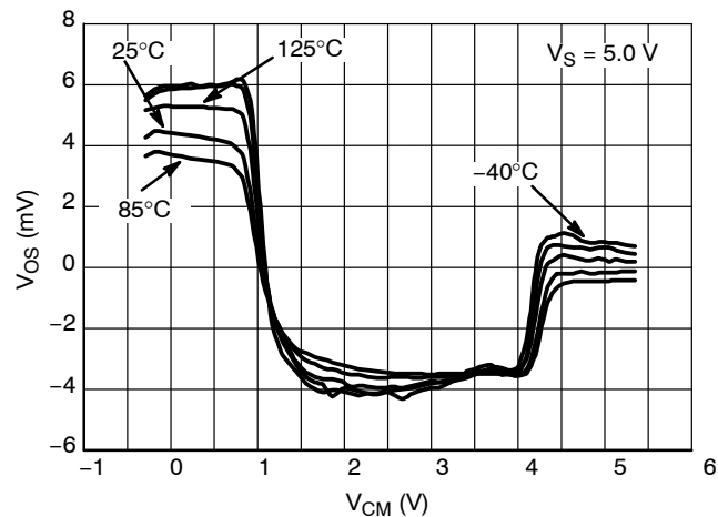
Figure 26. Offset Voltage vs. Common Mode Range V_{DD} 5.0 V
