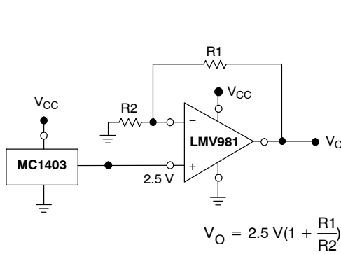
Figure 27. Voltage Reference
