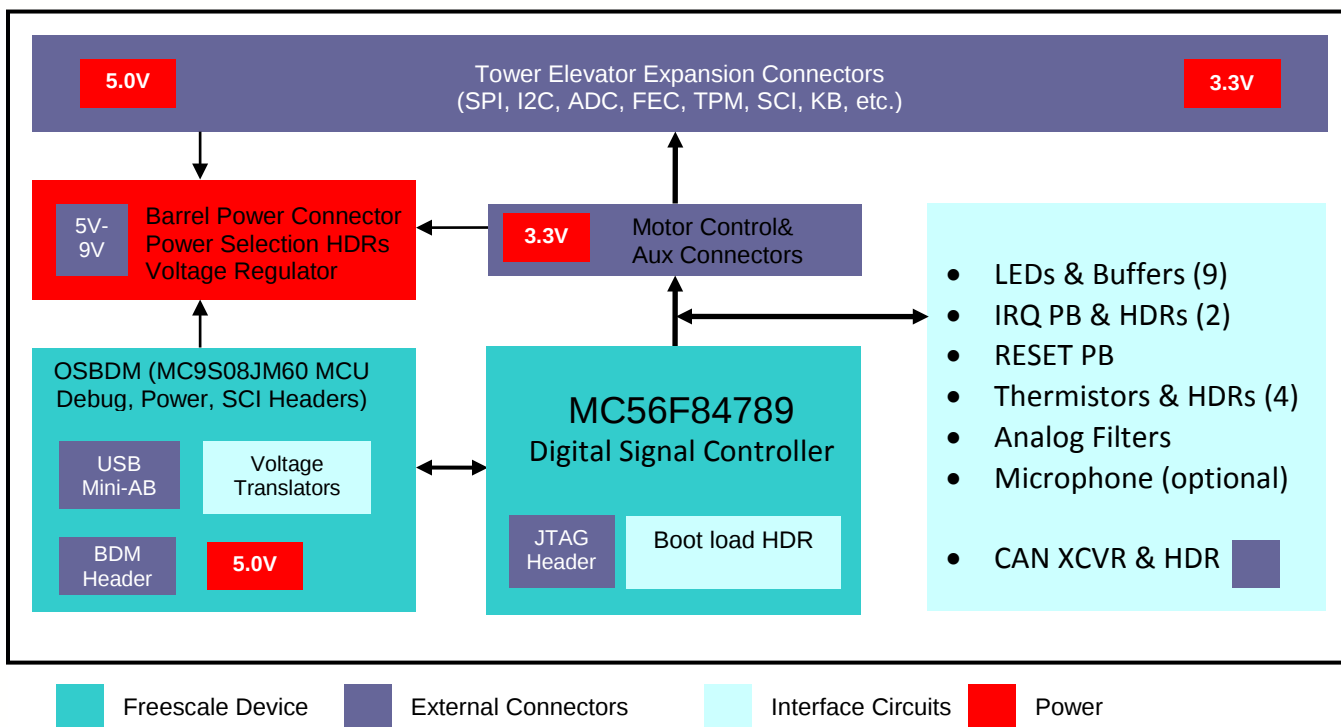
Figure 1. TWR-56F8400 Block Diagram
