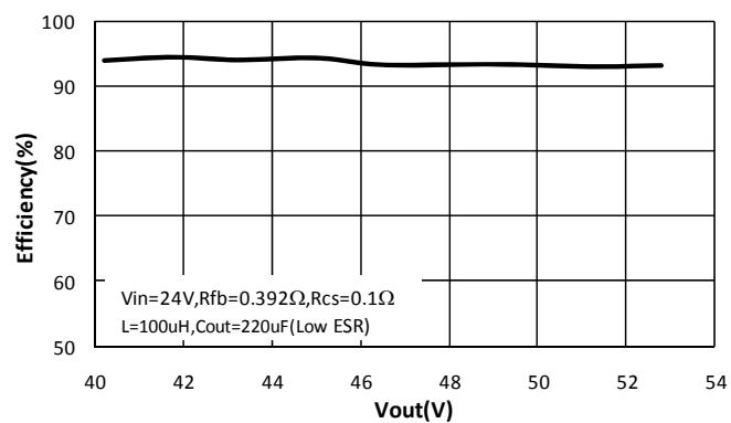
Figure 9. V_{out} & Efficiency
