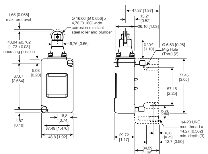
Figure 19. 206LS1 Dimensions
