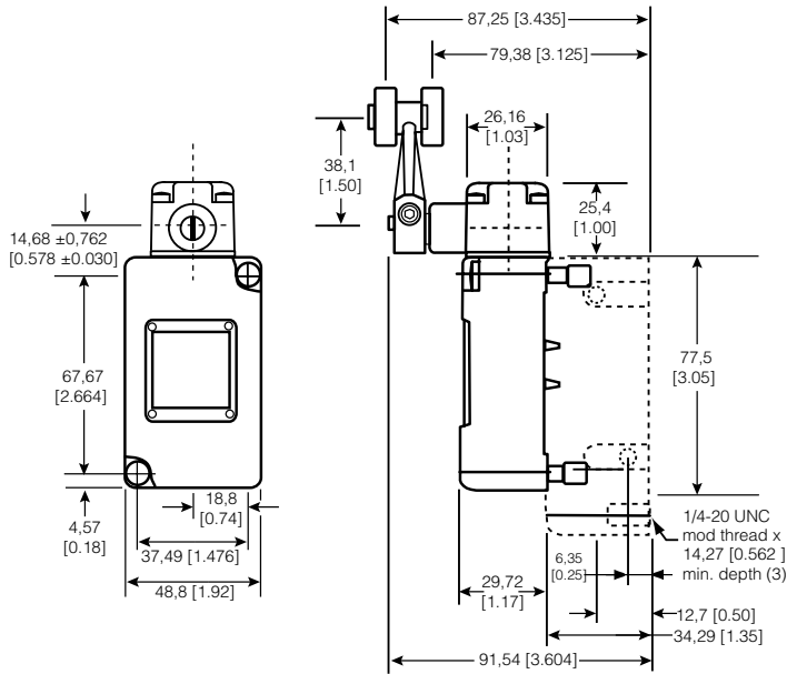
Figure 13. 201LS3 Dimensions
