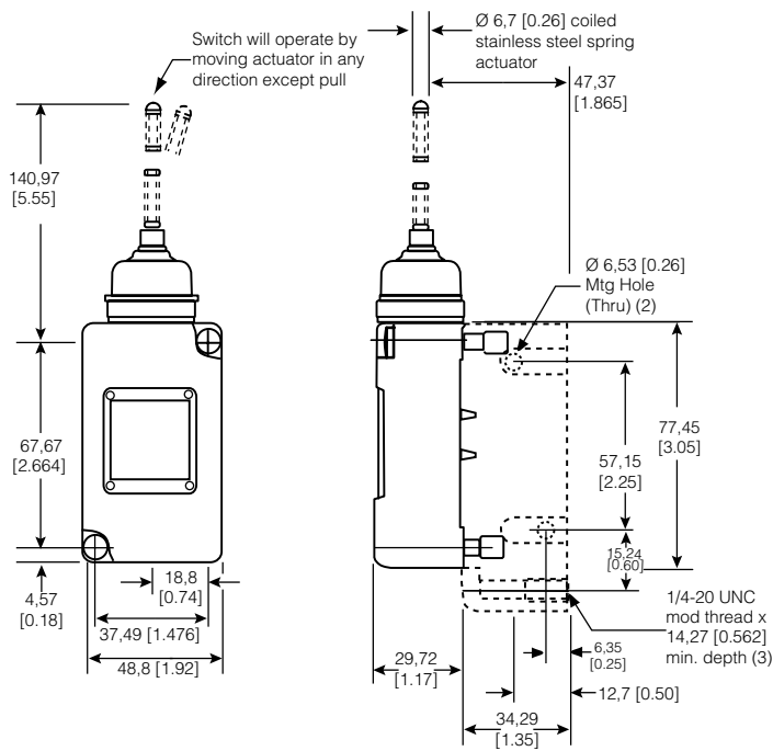
Figure 23. 208LS152 Dimensions
