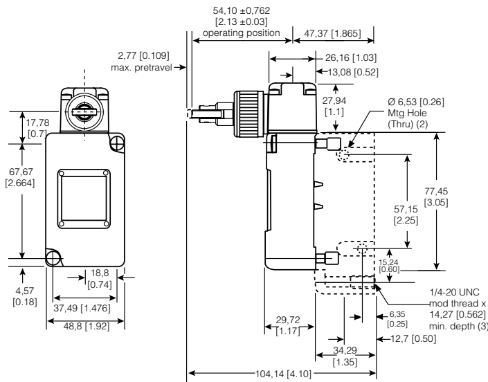
Figure 16. 203LS1 Dimensions
