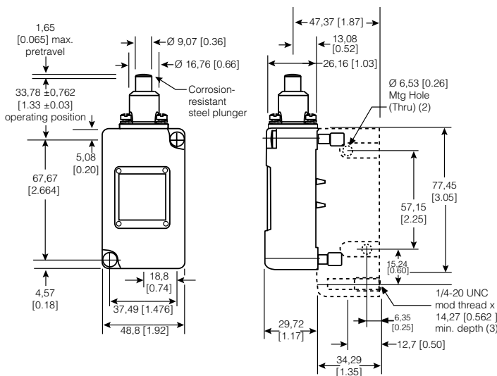
Figure 16. 203LS1 Dimensions
