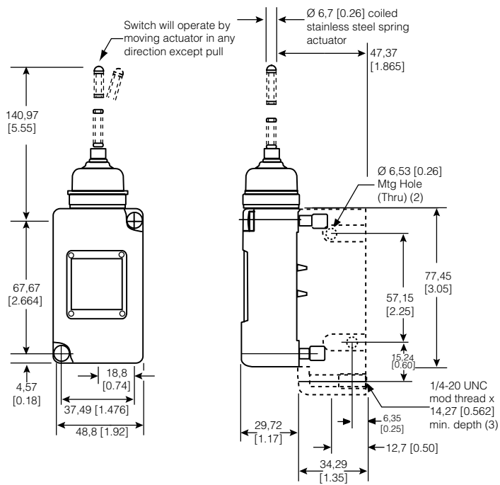
Figure 23. 208LS152 Dimensions
