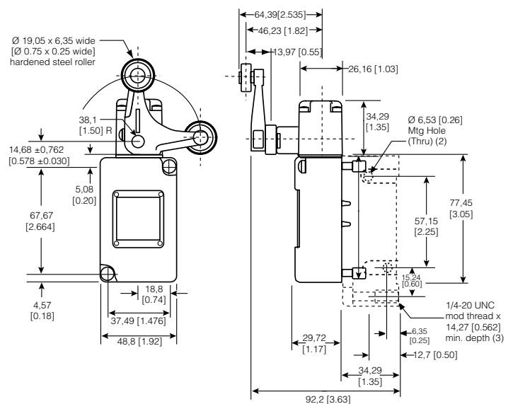
Figure 19. 206LS1 Dimensions
