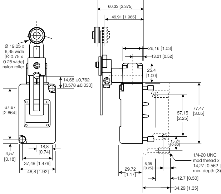
Figure 13. 201LS3 Dimensions
