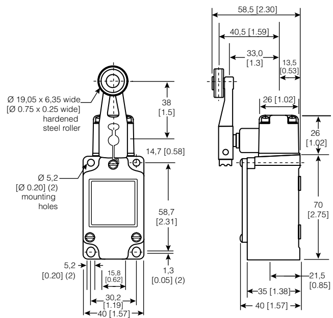
Figure 27. 2LS1-4 Dimensions
