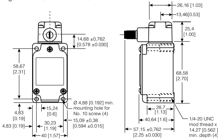
Figure 2. 1LS3 Dimensions
