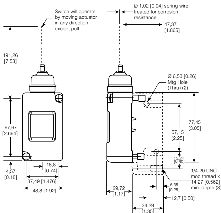
Figure 22. 208LS125 Dimensions
