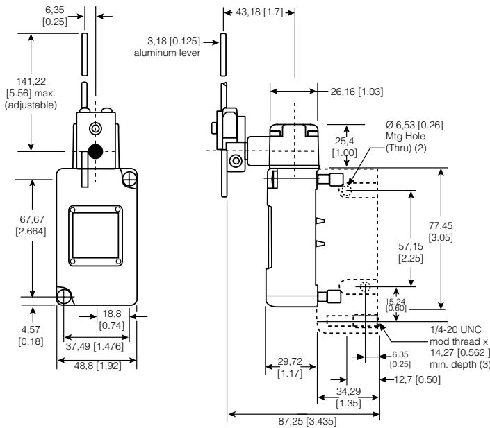
Figure 15. 202LS1 Dimensions
