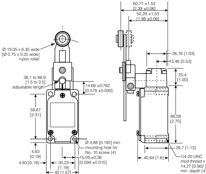
Figure 3. 1LS10 Dimensions
