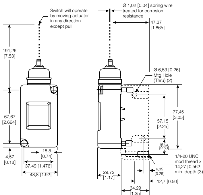
Figure 22. 208LS125 Dimensions
