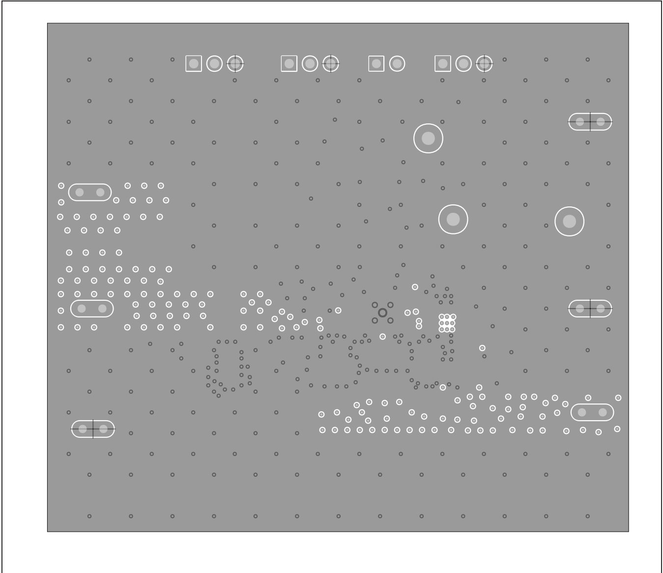
MAX20079 EVKIT Layout Internal 2
