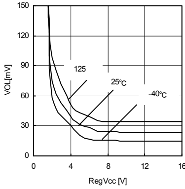
Fig. 11 Charge Pump NMOS On Resistance
