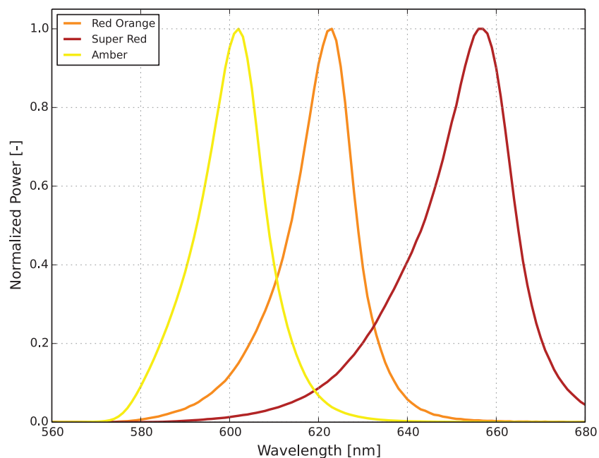
Figure 1. Typical normalized power vs. wavelength for SignalSure 75 at 20ms MP, 75mA, T_j=25^{\circ}\text{C} .
