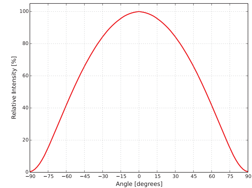
Figure 5. Typical radiation pattern for SignalSure 75 at 20ms MP, 75mA.
