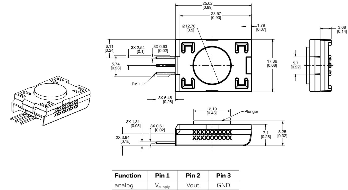
Figure 3. Mounting Dimensions (For reference only: mm/in.)
