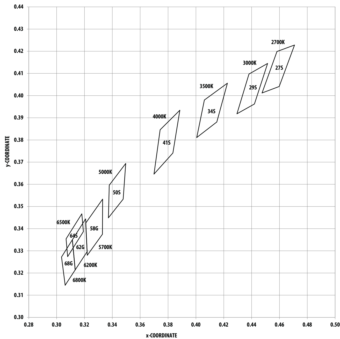
Figure 2: Chromaticity Diagram
