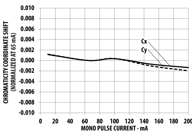
Figure 8: Chromaticity Coordinate Shift vs. Mono Pulse Current for 4000K
