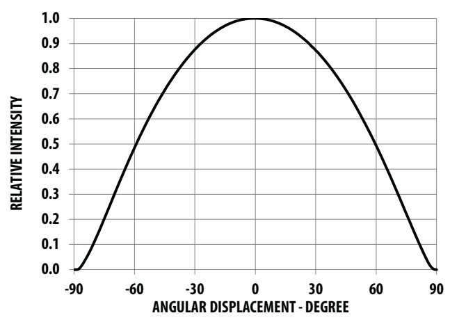
Figure 6: Radiation Pattern
