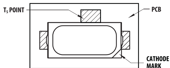
Figure 21: Solder Point Temperature on the PCB
