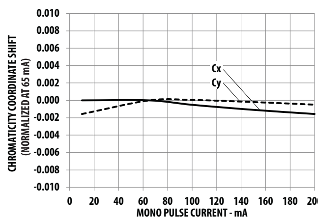
Figure 7: Chromaticity Coordinate Shift vs. Mono Pulse Current for 3000K
