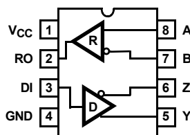
ISL83488, ISL83490 TOP VIEW
