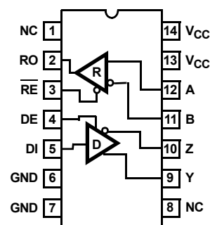
ISL83491 TOP VIEW
