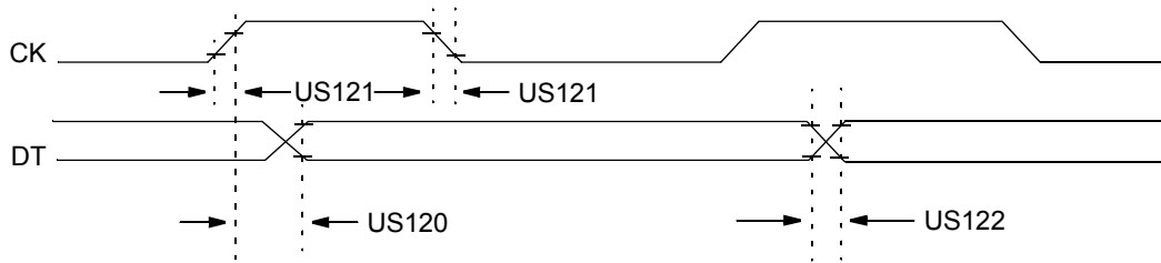
Figure 38-14. EUSART Synchronous Transmission (Master/Slave) Timing
