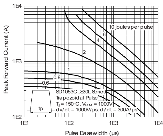
Fig. 36 - Maximum Total Energy Loss Per Pulse Characteristics
