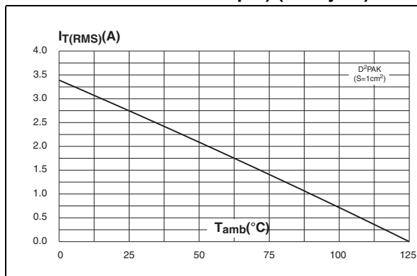
Figure 3. D 2 PAK RMS on-state current versus ambient temperature (printed circuit board FR4, copper thickness: 35 \mu m) (full cycle)
