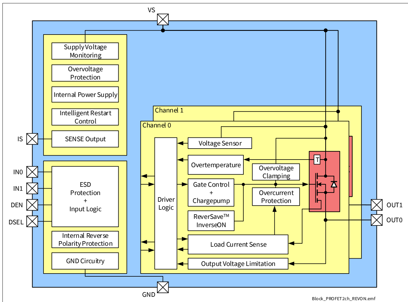
Figure 2 Block Diagram of BTS7008-2EPA
