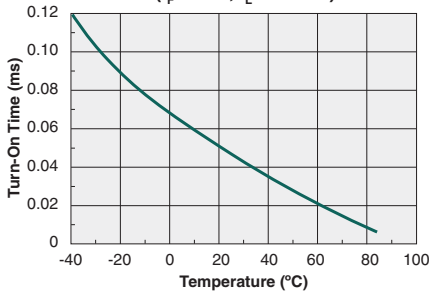
Typical Turn-On Time vs. Temperature ( I_F=5mA, I_L=200mA )
