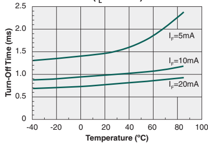
Typical Turn-Off Time vs. Temperature ( I_L=200mA )
