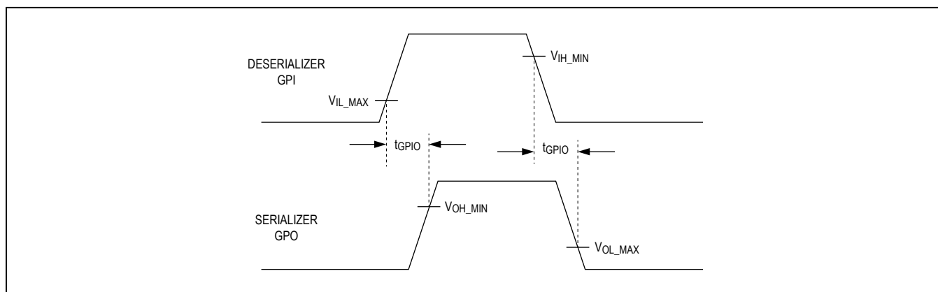
Figure 9. GPI-to-GPO Delay
