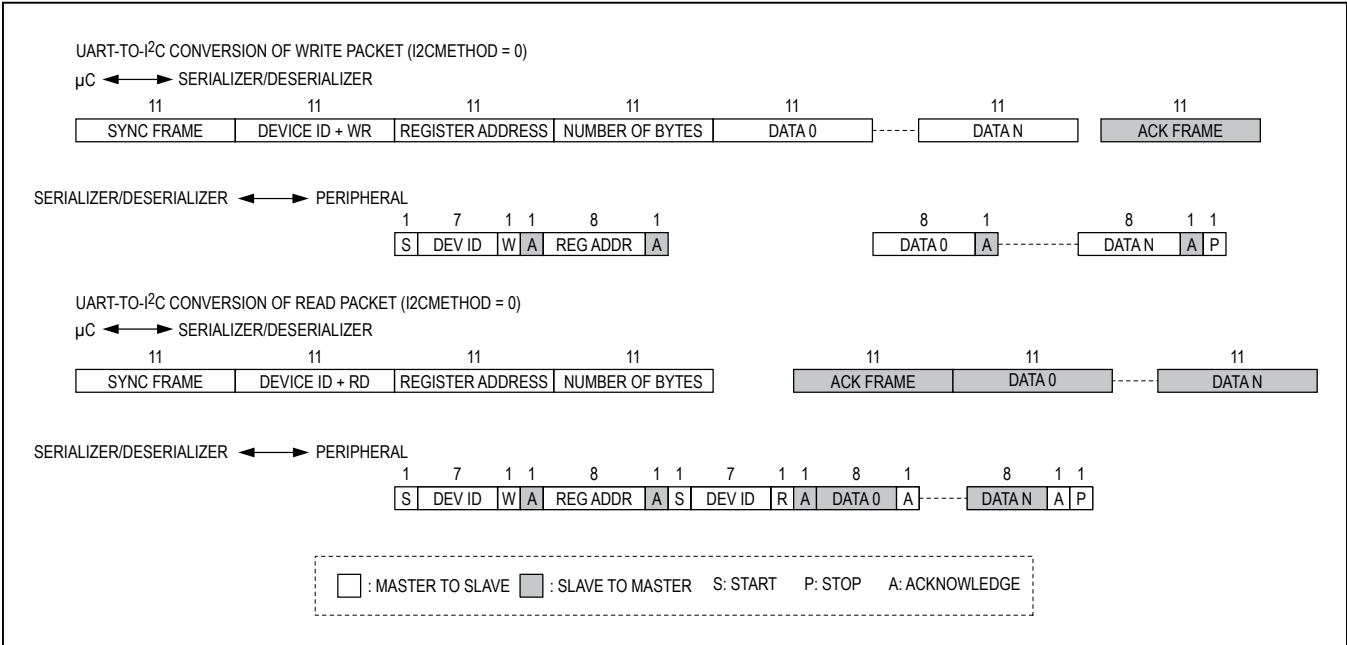
Figure 25. Format Conversion Between GMSL UART and I²C with Register Address (I2CMETHOD = 0)
