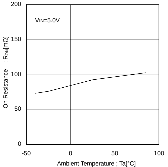
Figure 13. On Resistance
