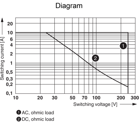
Interrupting rating
