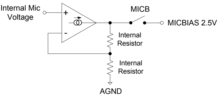
Figure 18. Mic Bias
