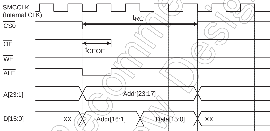
Figure 10-2 Asynchronous Read
