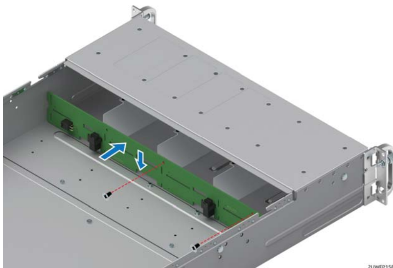
Figure 47. 3.5" backplane placement
