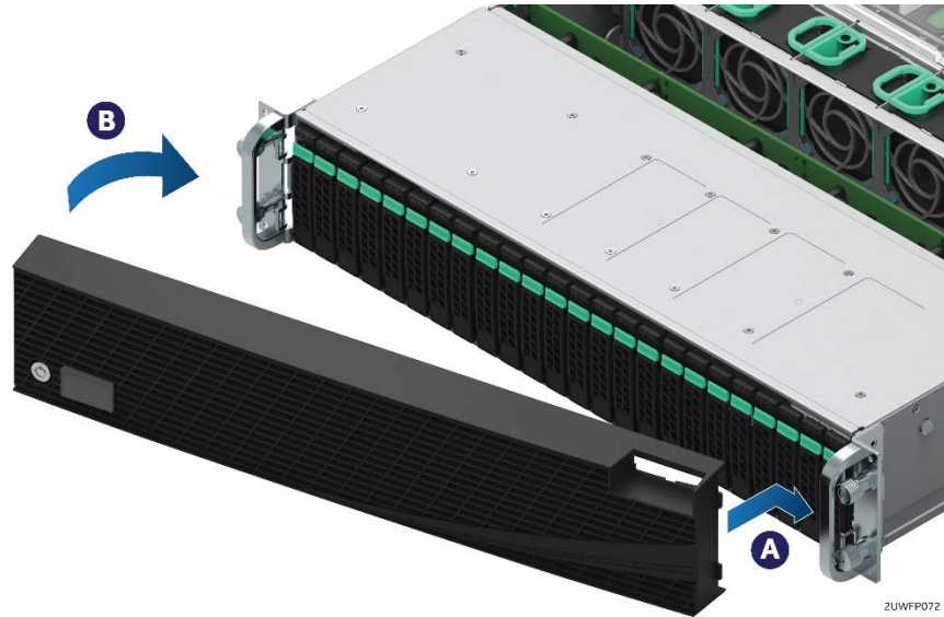
Figure 15. Concept Reference Design – Front Bezel Installation
