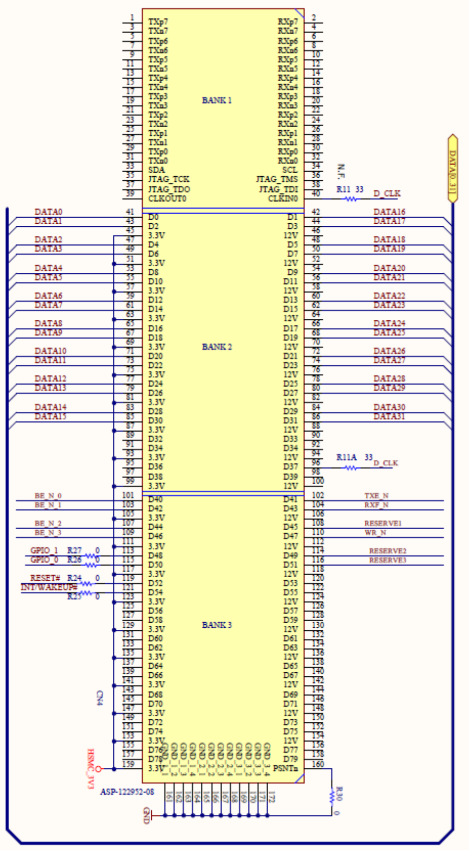
Figure 3-3 Schematics: HSMC_UMFT602A
