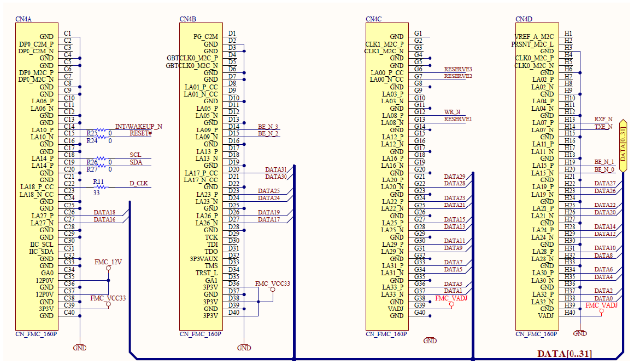
Figure 3-4 Schematics: FMC_UMFT602X
