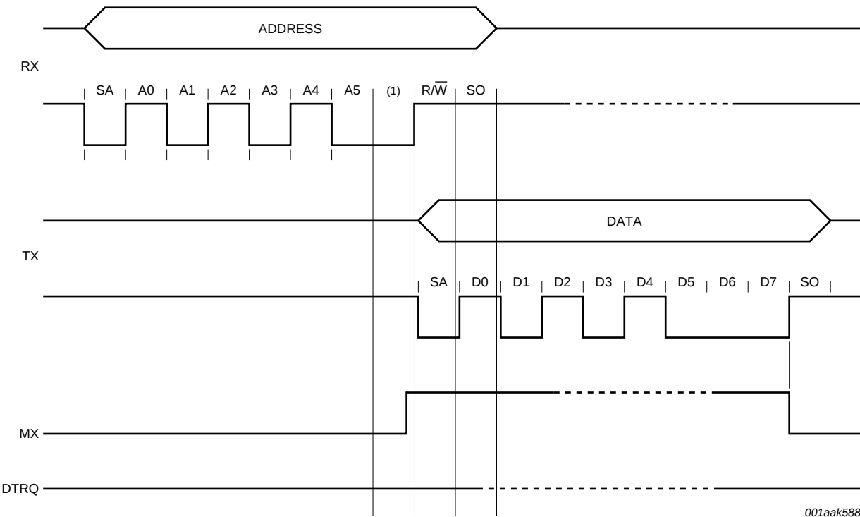
Fig 15. UART read data timing diagram
