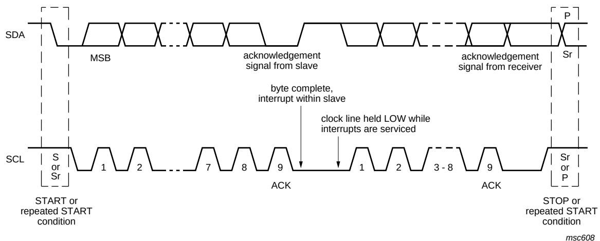
Fig 21. Data transfer on the I 2 C-bus
