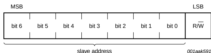
Fig 22. First byte following the START procedure
