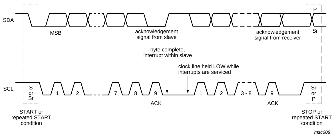
Fig 21. Data transfer on the I²C-bus
