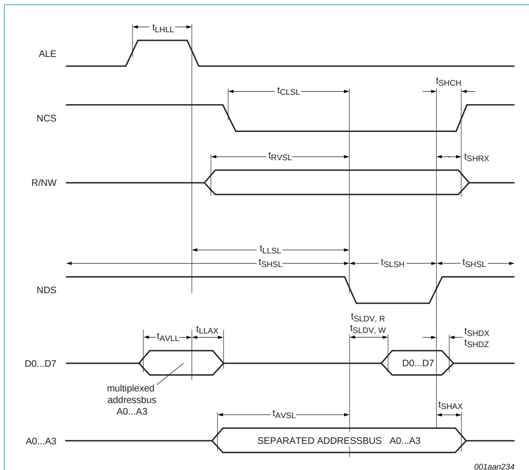
Fig 43. Timing diagram for common Read/Write strobe
